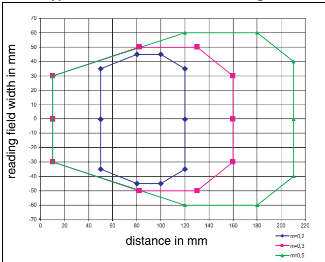
BCL 34 type L with 800scans/s with heating
