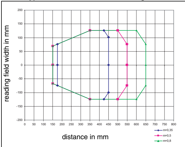
BCL 34 type L with 800scans/s with heating
