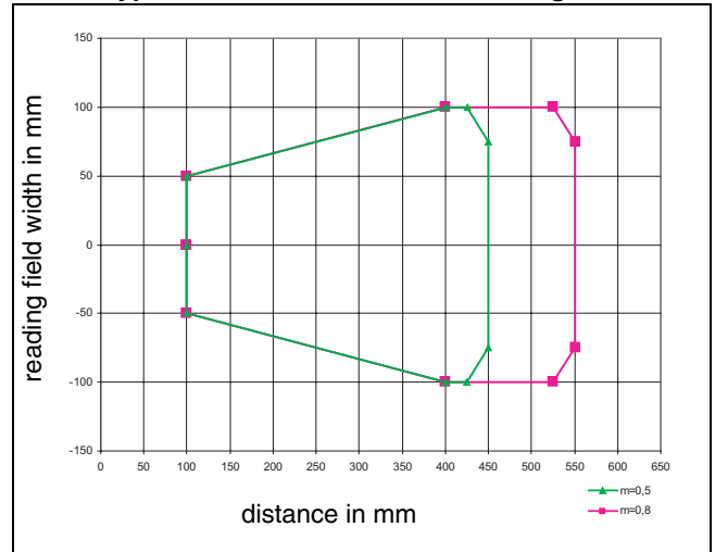
BCL 34 type J with 1000scans/s with heating 1)
